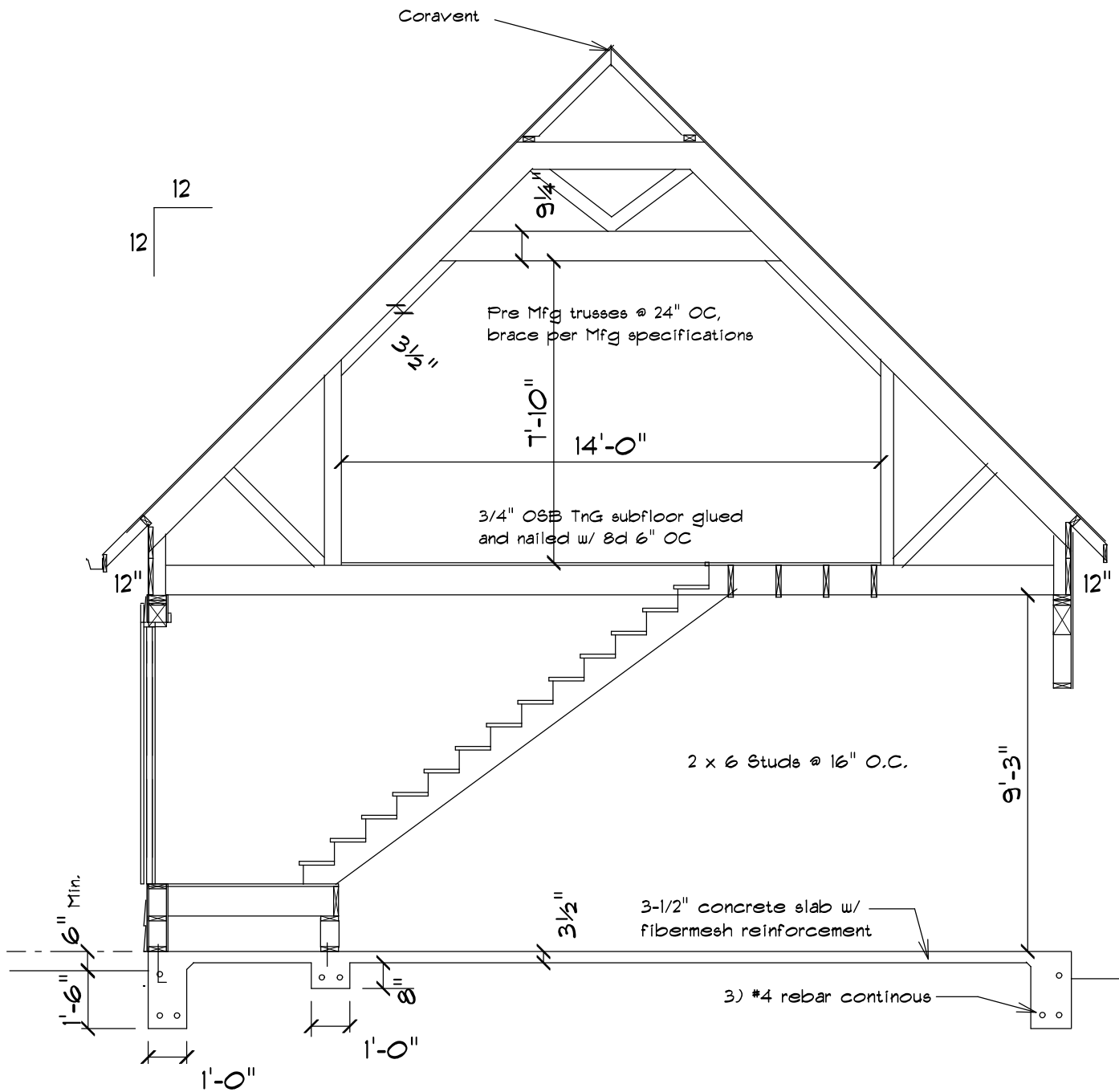
Gable Style Room in the Roof Cross Section
